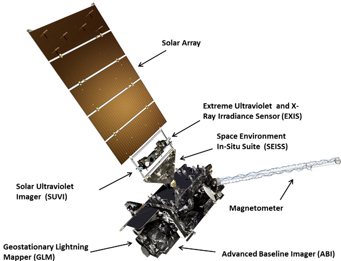
Fig. 1. The GOES-R spacecraft and instruments.
