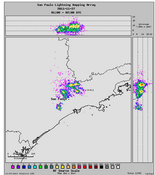
Fig. 9. São Paulo Lightning Mapping Array (SPLMA) station showing the VHF (Channel 8, 162 MHz) ground plane antenna, sensor electronics and computer package (lower left). Plot with horizontal and vertical projections of 1-hour source density for 0100–0200 UTC on 27-Nov-2011 (lower right) encompassing the LIS overpass 0131–0135 UTC and WWLLN observations (above).
