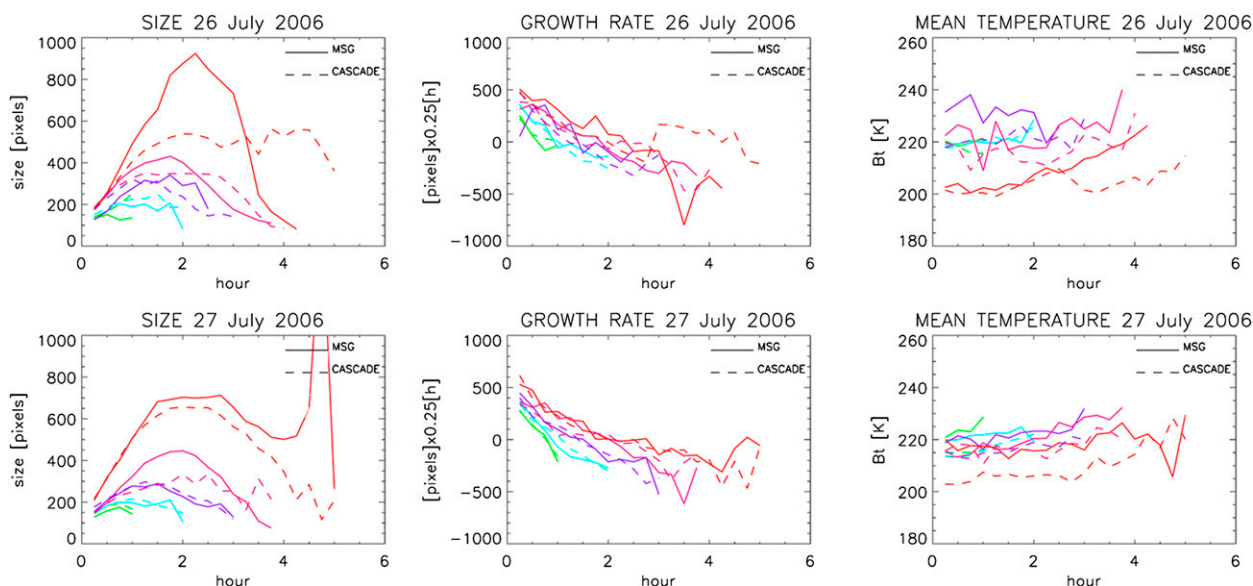
FIG. 5. (left) Mean size (center) growth rate, and (right) mean temperature for the convective systems for (top) 26 and (bottom) 27 Jul 2006. Dashed lines represent UK UM–RTTOV simulation statistics, and green, light blue, purple, pink, and red represent the systems living up to 1, 2, 3, 4, and >4 h, respectively.
