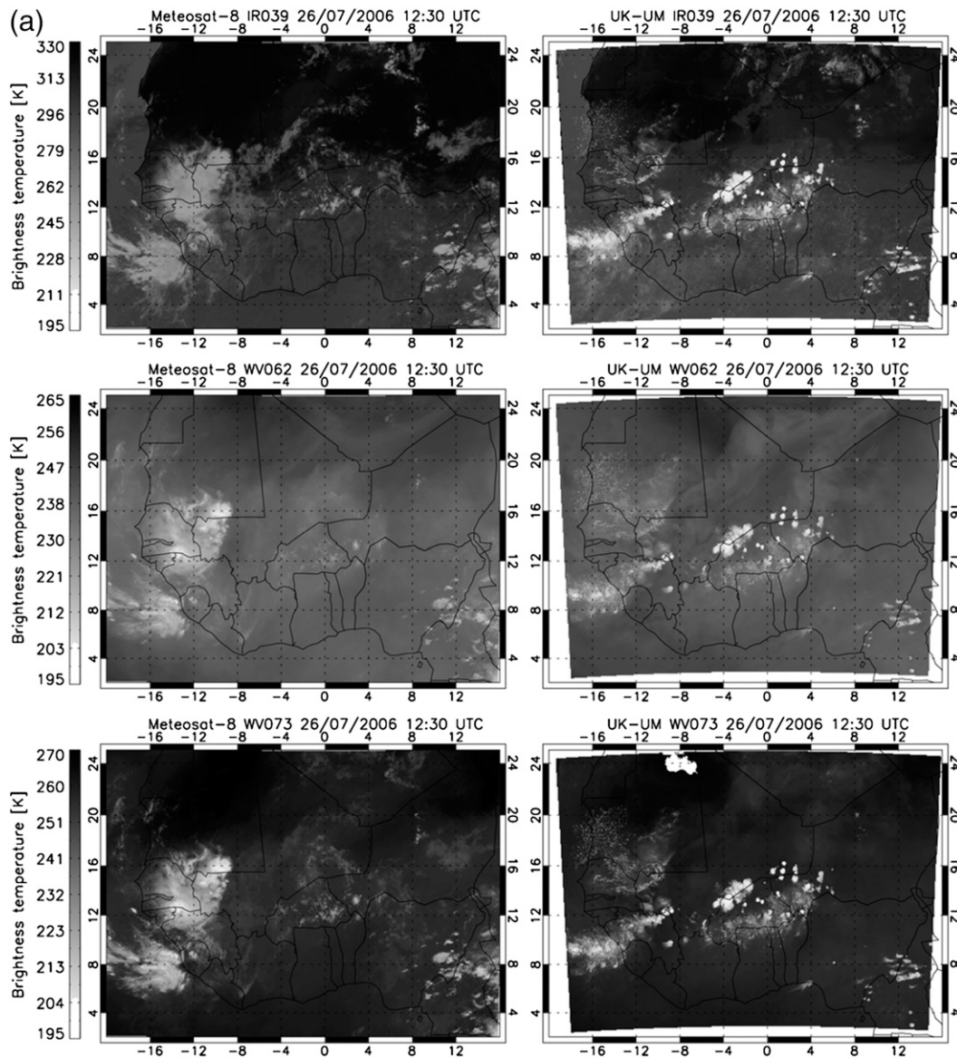
FIG. 1. (left) Real SEVIRI-MMSG imagery and (right) simulated SEVIRI for (a) channels (top) 3.9, (middle) 6.2, and (bottom) 7.3 \mu\text{m} , (b) channels (top) 8.7 and (bottom) 10.8 \mu\text{m} , and (c) channels (top) 12 and (bottom) 13.4 \mu\text{m} at 1230 UTC 26 Jul 2006.
