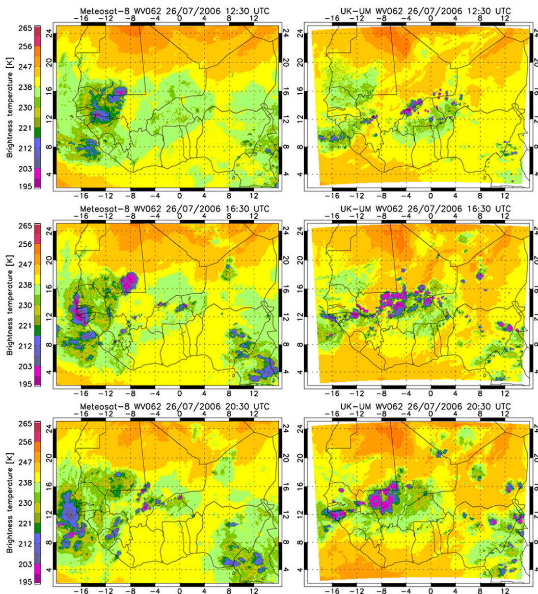
FIG. 3. (left) Real MSG measurements and (right) UK UM-RTTOV simulations at (top) 1230, (middle) 1630, and (bottom) 2030 UTC 26 Jul 2006. Notice that in the areas away from deep convection, brightness temperatures are generally warmer than in reality.
