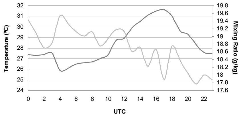
Figure 3 – Hourly temperature (black) and mixing ratio (gray) for 2010/03/10.
