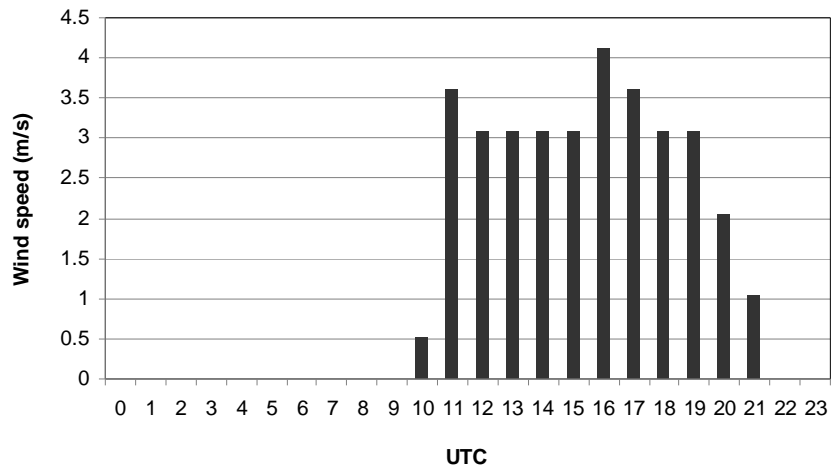
Figure 2 – Hourly wind speed for 2010/03/10.
