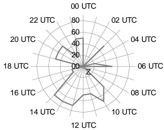
Figure 1 – Hourly wind direction for 2010/03/10.
