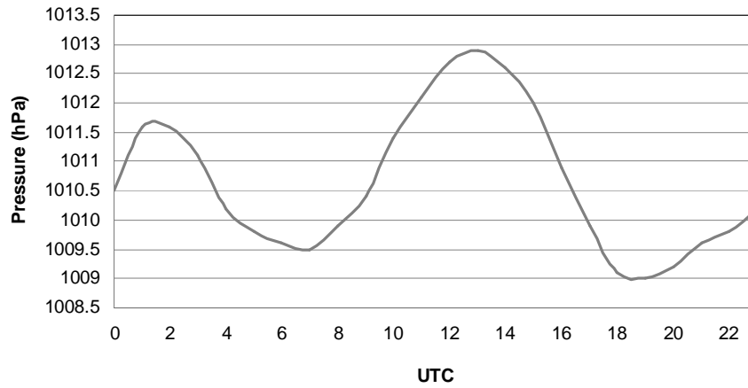
Figure 4 – Hourly sea level pressure for 2010/03/10.
